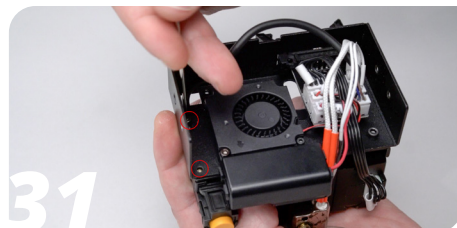
31 Add the screws holding the bed probe and fasten them.
