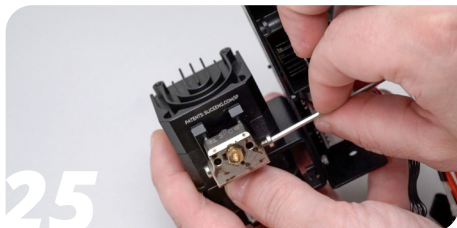
25 Remove the heater and thermistor retention screw with a 2 mm hex key.
