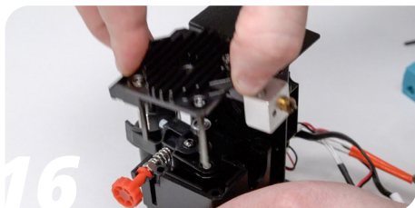
Remove the hotend heatsink.
