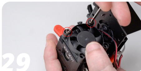
29 Add the hotend heatsink fan and to the top fasten M3x12 SHCS screws with a 2.5 mm hex key.
