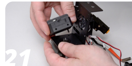
Add the extruder motor and the extruder to the carriage.
