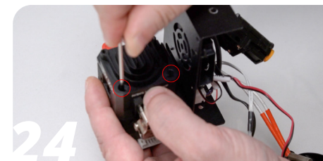
Fasten the two M3 screws at the bottom using a 2 mm hex key.
