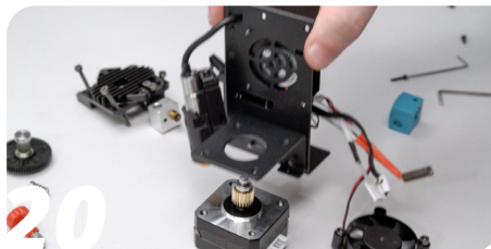
Remove the rest of the extruder and the motor from the carriage.
