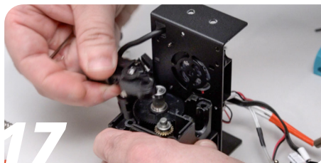
Remove the extruder tensioning assembly.
