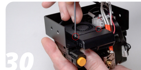
30 Add the two screws holding the fan shroud and fasten them.
