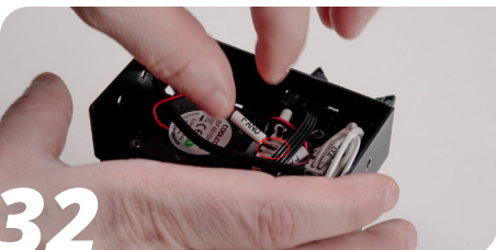
32 Disconnect the part cooling fan.
