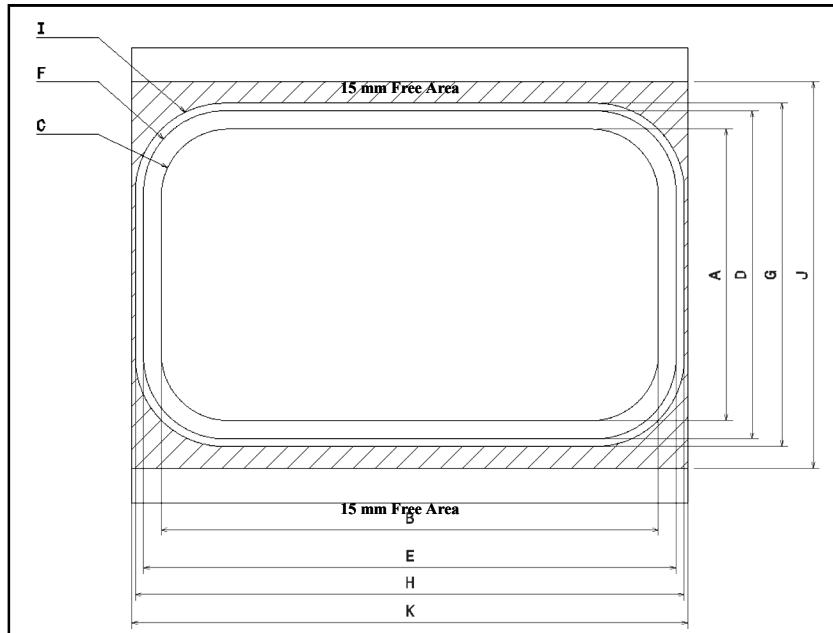
Window Dimensions Front View In Millimeters
