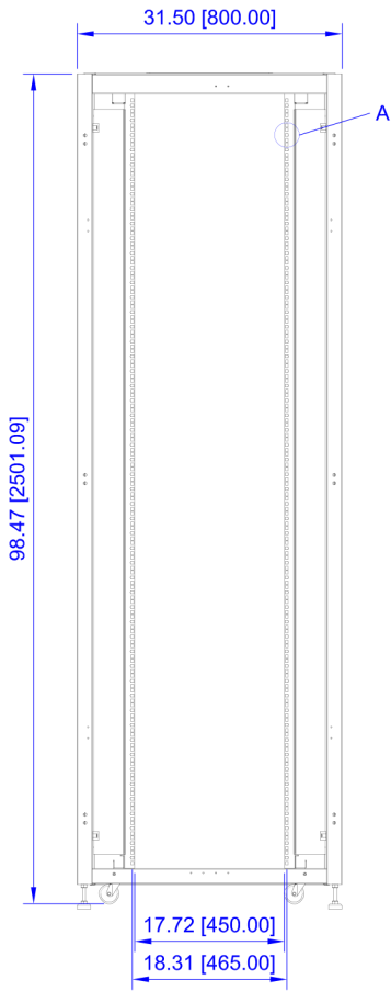
FRONT VIEW (NO DOOR)
