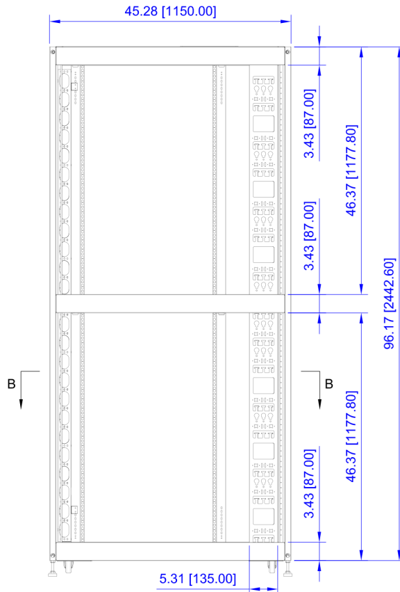
SIDE VIEW (NO SIDE PANELS)
