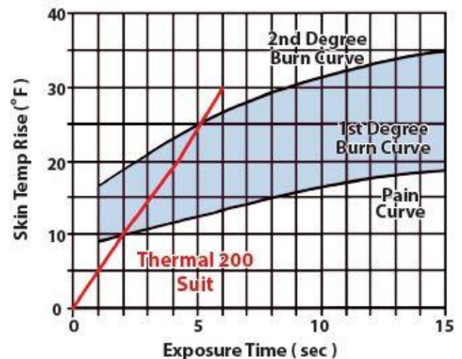
Thermal Performance of Thermal 200 Suit Against Hot Oil at 752°F (400°C)
