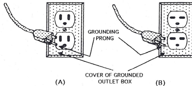
FIGURE 1 GROUNDING METHODS
