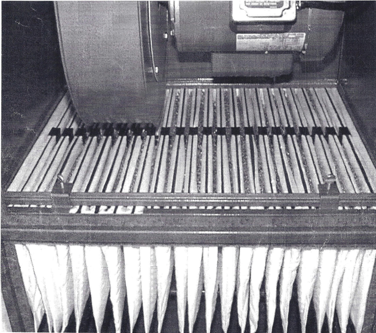
Example Placement and Installation Of Filter Bags And Brackets
