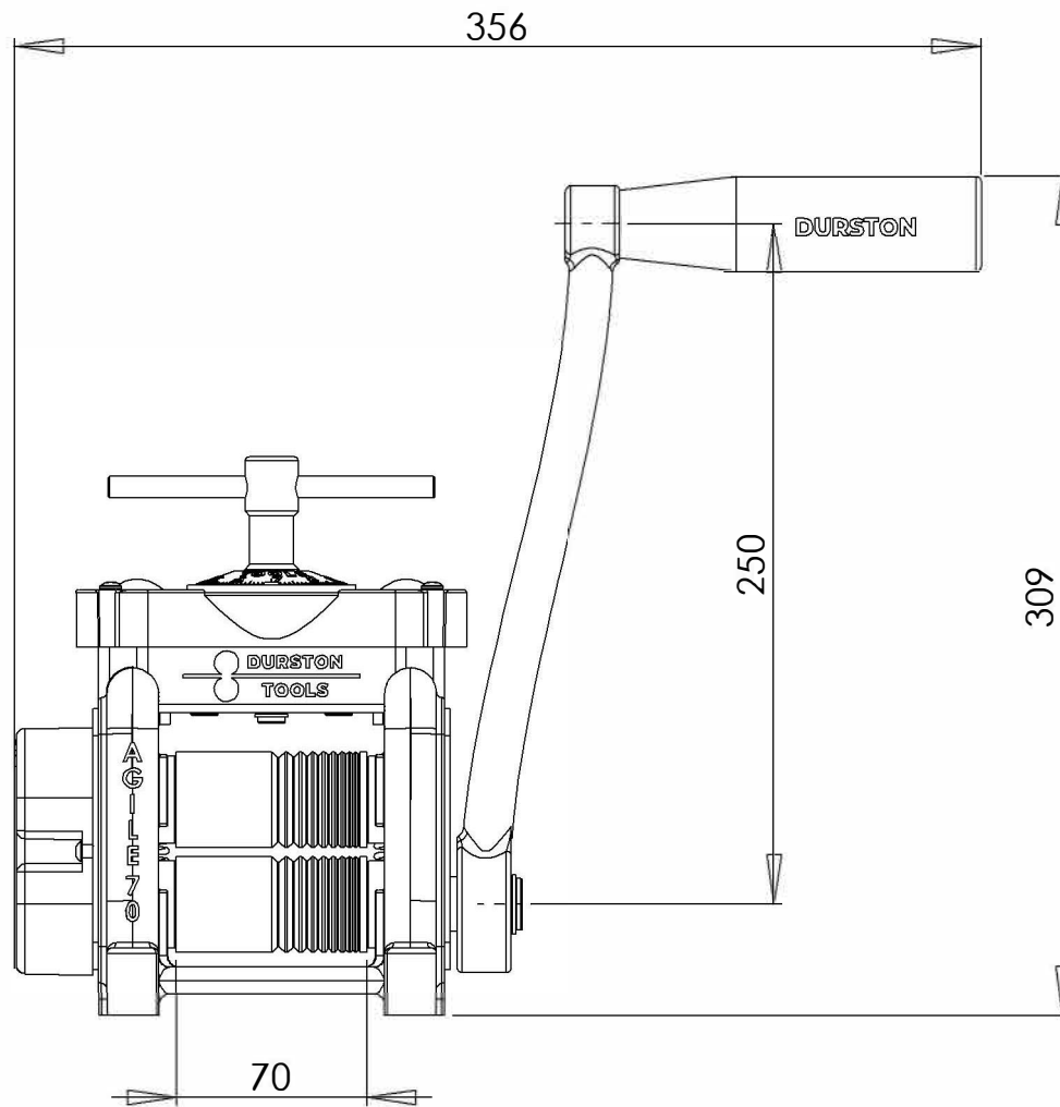
Agile 70 Rolling Mill SKU: 1058 Dimensions is MM
