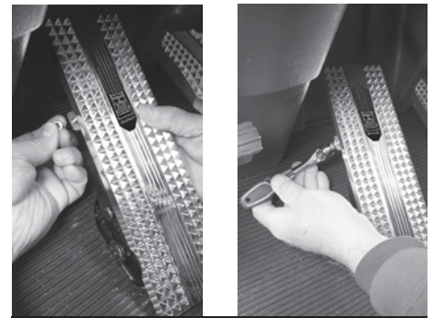
PHOTO 12 — BRAKE PEDAL
