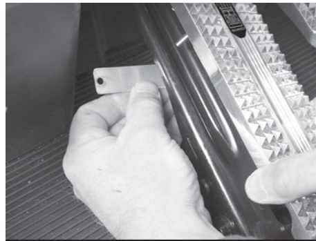
PHOTO 11 — BRAKE PEDAL
