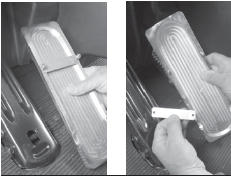
PHOTO 10 — BRAKE PEDAL
