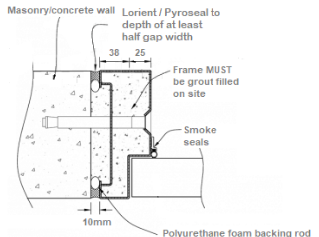
FRAME PROFILE G
