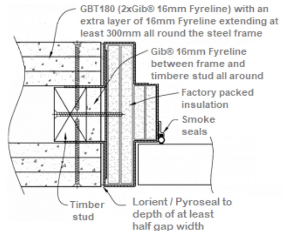
FRAME PROFILE D SHOWN (ONLY AVAILABLE FRAME PROFILE)
