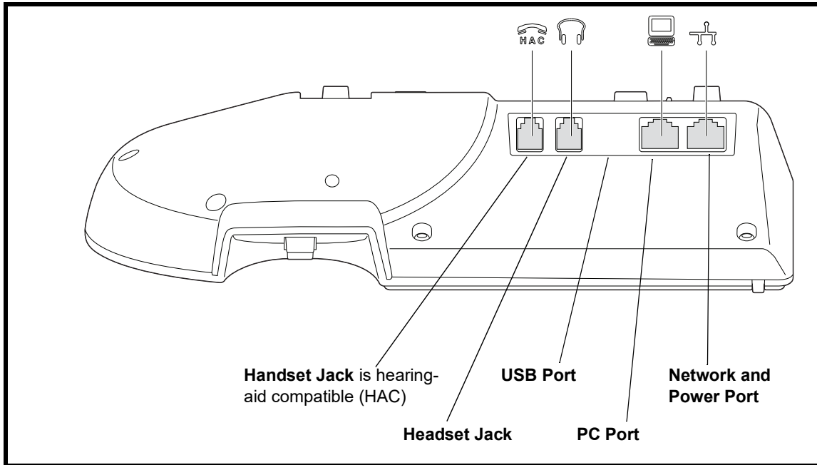
Figure 2: Ports on the Back of the IP Phone 485g
