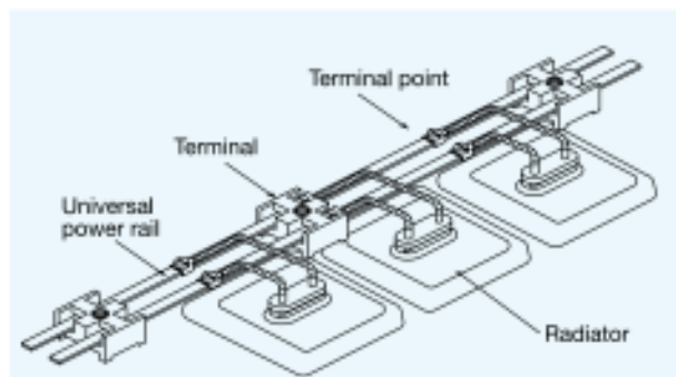
Figure 13: Rail wiring
