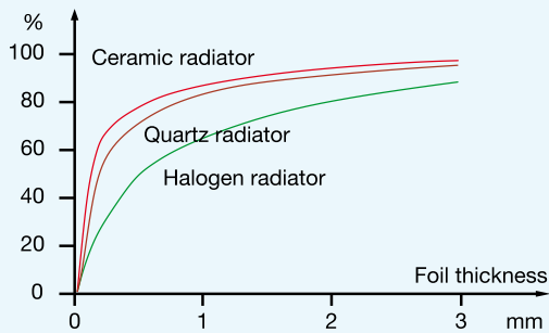
Figure 20: Absorption in transparent foils
