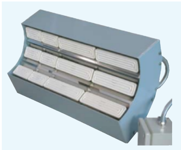
Figure 26: Roller heating
