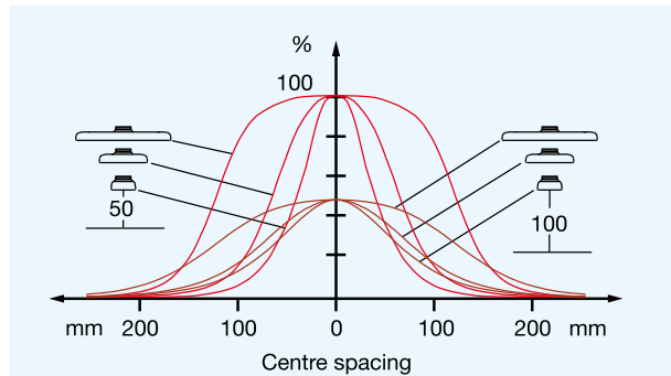
Figure 14: Spatial radiation distribution
