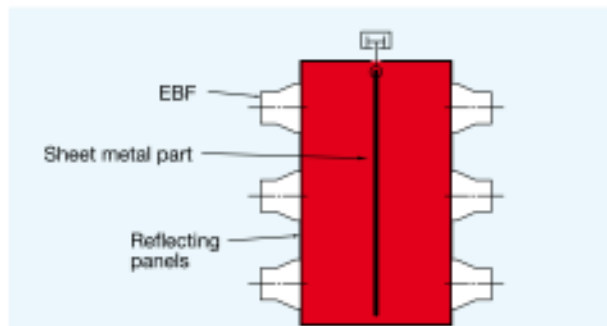
Figure 11: Radiation tunnel with several EBF systems
