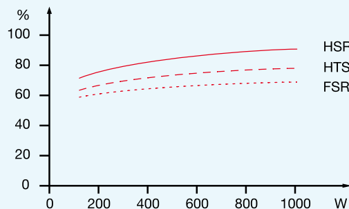
Figure 21: Efficiencies dependent on the power
