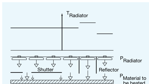
Figure 17: Power adjustment with reflector and shutter
