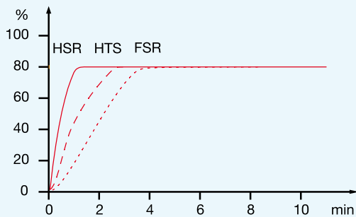
Figure 19: Power in controlled operation
