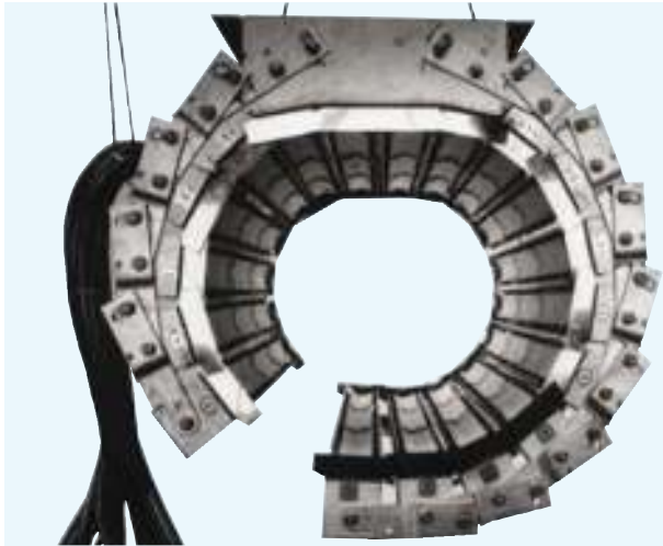
Figure 28: Heating head for heating GRP pipes
