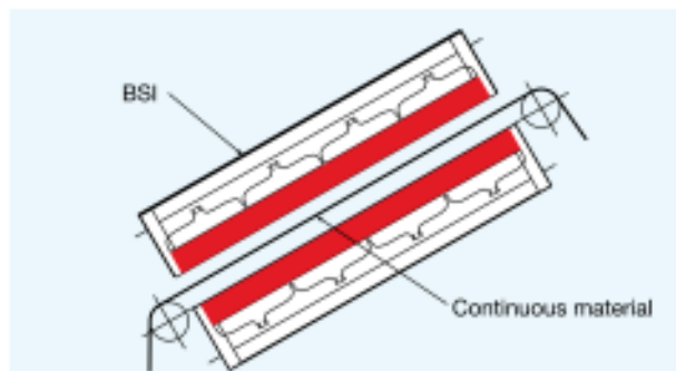
Figure 12: Heating a continuous material using 2 BSI systems
