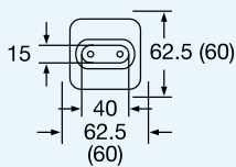
Figure 32: Mounting dimensions and radiator dimensions ( ) in mm
