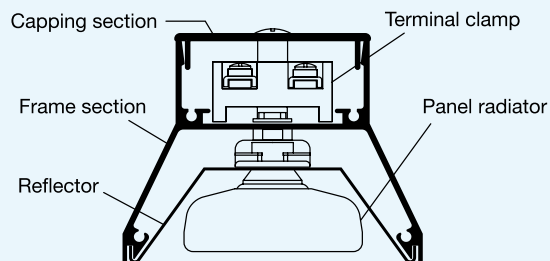
Fig. 77: Cross-section through an EBF construction element
