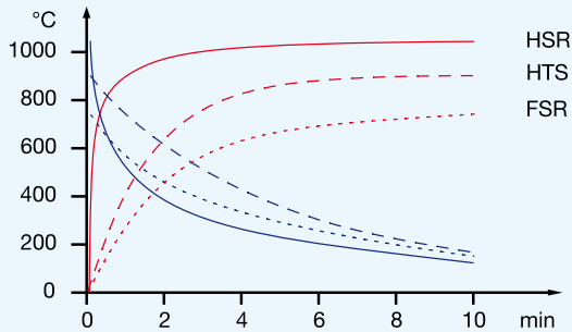
Figure 18: Heating-up and cooling performance
