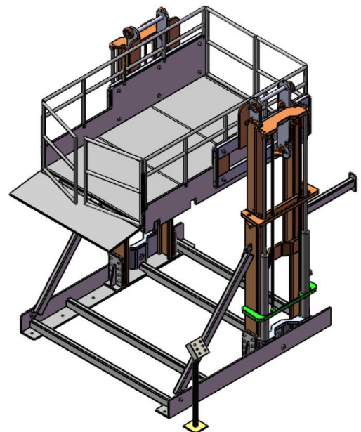
RAISED POSITON
