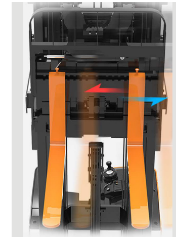
Maximum reach distance up to 1080 mm | 42.5"
