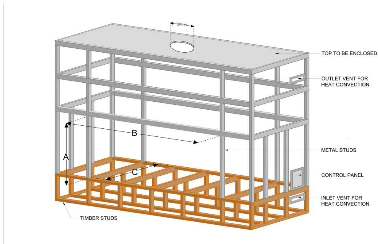
Figure 1.9 (Metal framing)
