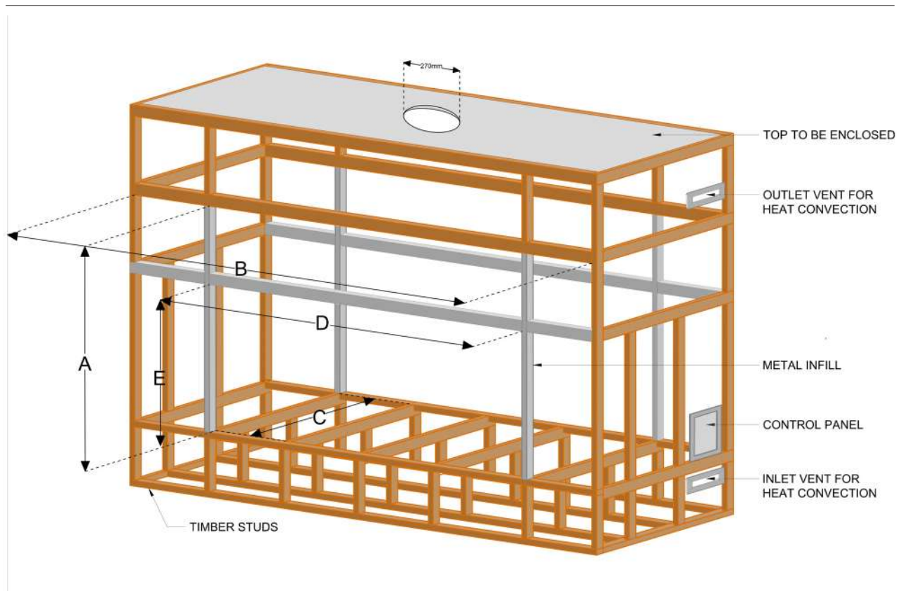
Figure 1.8 (Timber framing)
