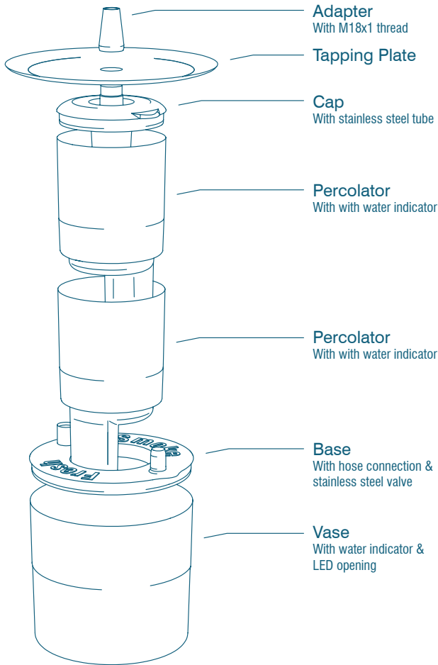
Mounting of the lowest Percolator Align the lowest Percolator to the text as shown
