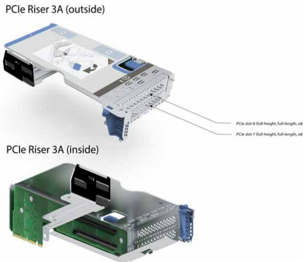
Figure 10 Riser Card 3A
