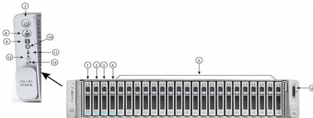
Figure 2 Chassis Front View (UCSC-C245-M8SX)
