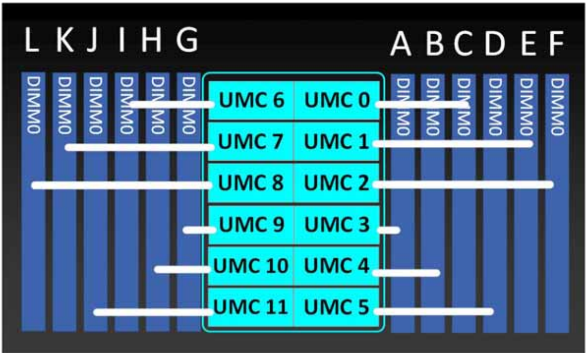
Figure 4 12-Channel Memory Organization
