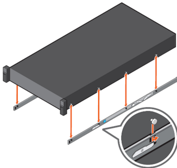
Figure 42. Attach the inner rails to the system
