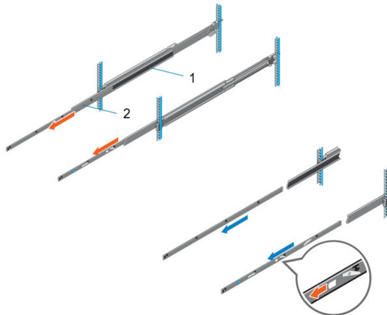
Figure 31. Pull out the intermediate rail
