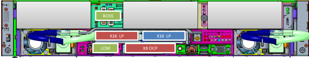
Figure 8. Rear view of the system with riser config 1: SAS/SATA SSD only or NVMe RAID (not direct attach)
