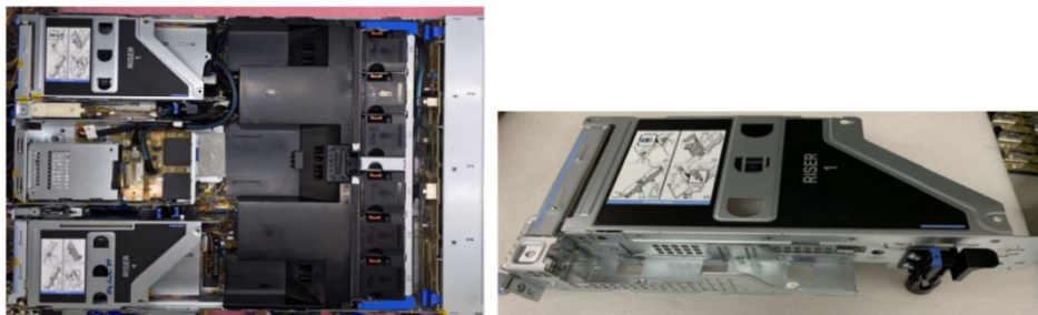
Figure 30. Shroud/HSK/Riser Cage
