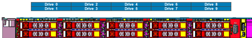
Figure 3. Front view of the system 10x 2.5-inch drives
