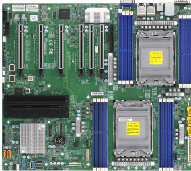
GPU Serverboard
