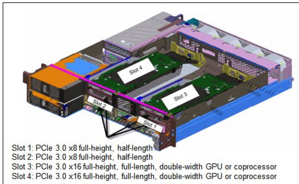
Figure 5. PCIe tray
