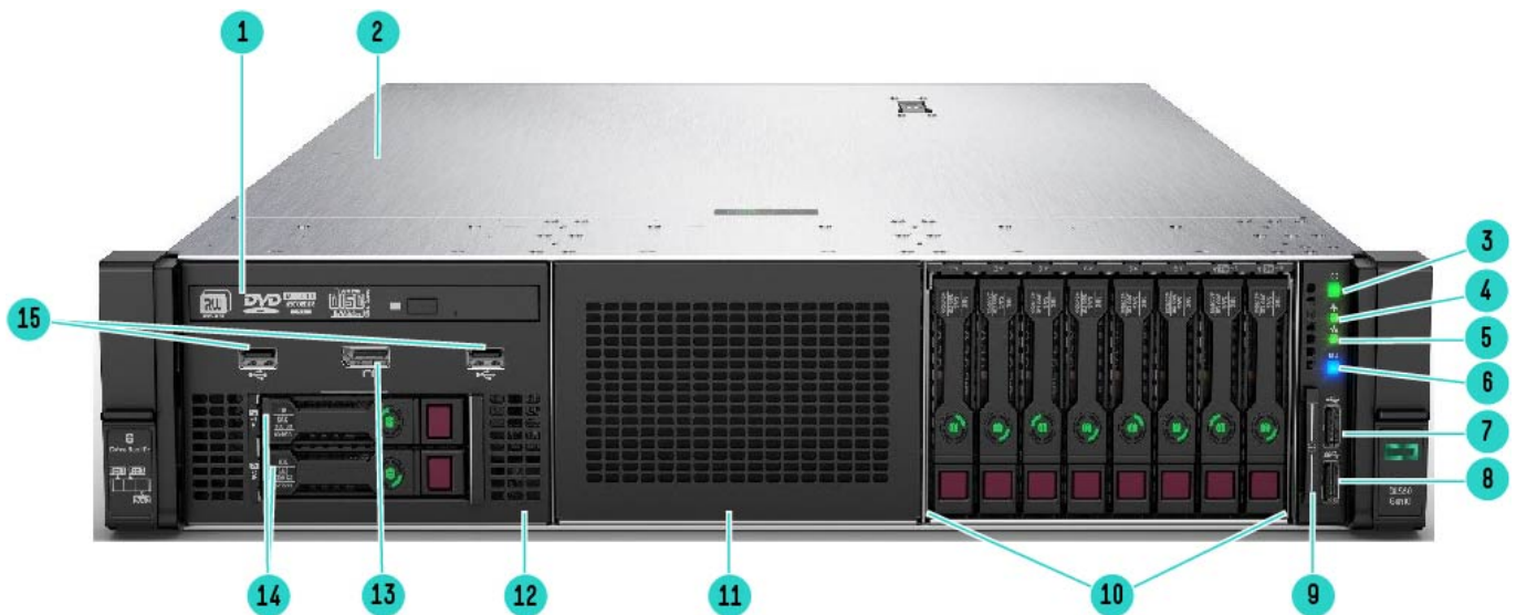
HPE ProLiant DL560 Gen10 Server - Front View
