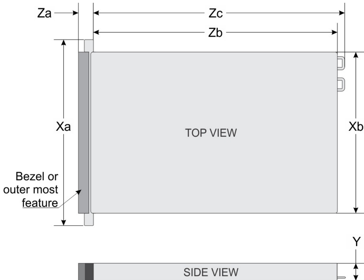
Figure 18. PowerEdge R450 Chassis dimensions
