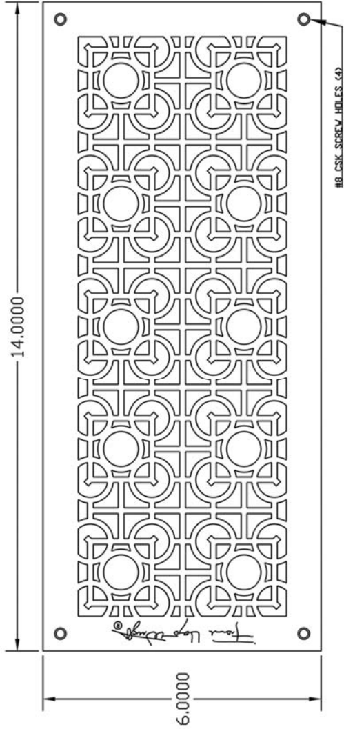
A PLAN SCALE 6" = 1'
