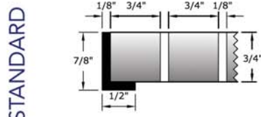
EC 300 A FRAME
