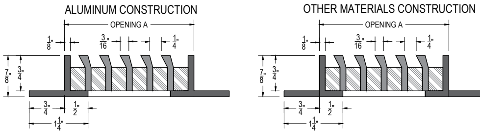
SECTION VIEW SCALE 1:1
