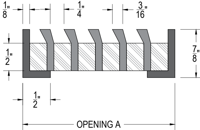
SECTION VIEW SCALE 1:1
