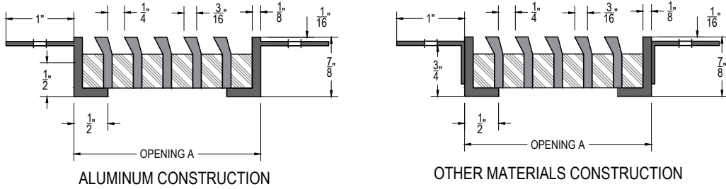
SECTION VIEW SCALE 1:2
