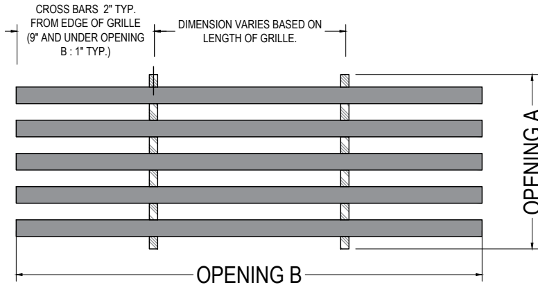
OPENING B PLAN VIEW SCALE 1:2
