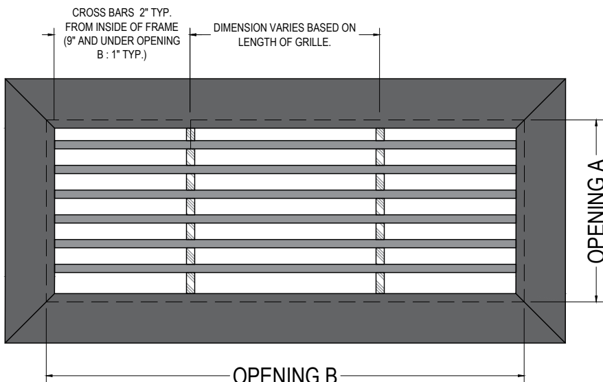
PLAN VIEW SCALE 1:2
