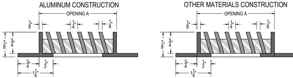
SECTION VIEW SCALE 1:1
