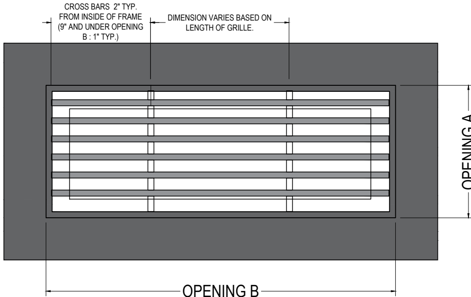
OPENING B PLAN VIEW SCALE 1:2
