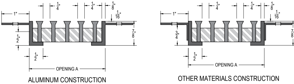
SECTION VIEW SCALE 1:2
