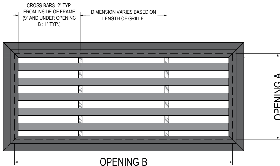
PLAN VIEW SCALE 1:2
