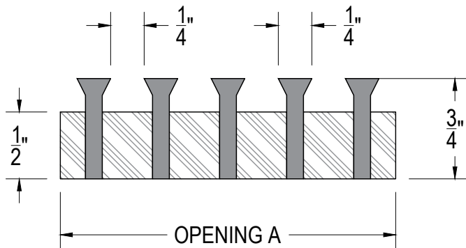
SECTION VIEW SCALE 1:1
