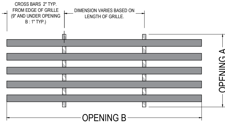
PLAN VIEW SCALE 1:2
