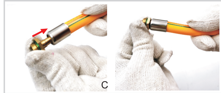
C : Thrust connector into hose
