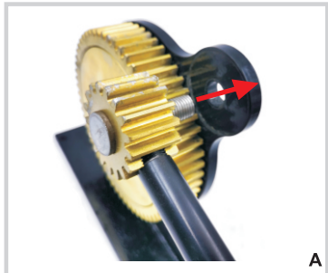
A: Thrust bolt into hole to mesh gears
