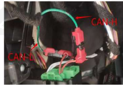
15. Our CAN-H cable is connected to the orange-grey cable and the CAN-L cable is connected to the orange-brown cable
