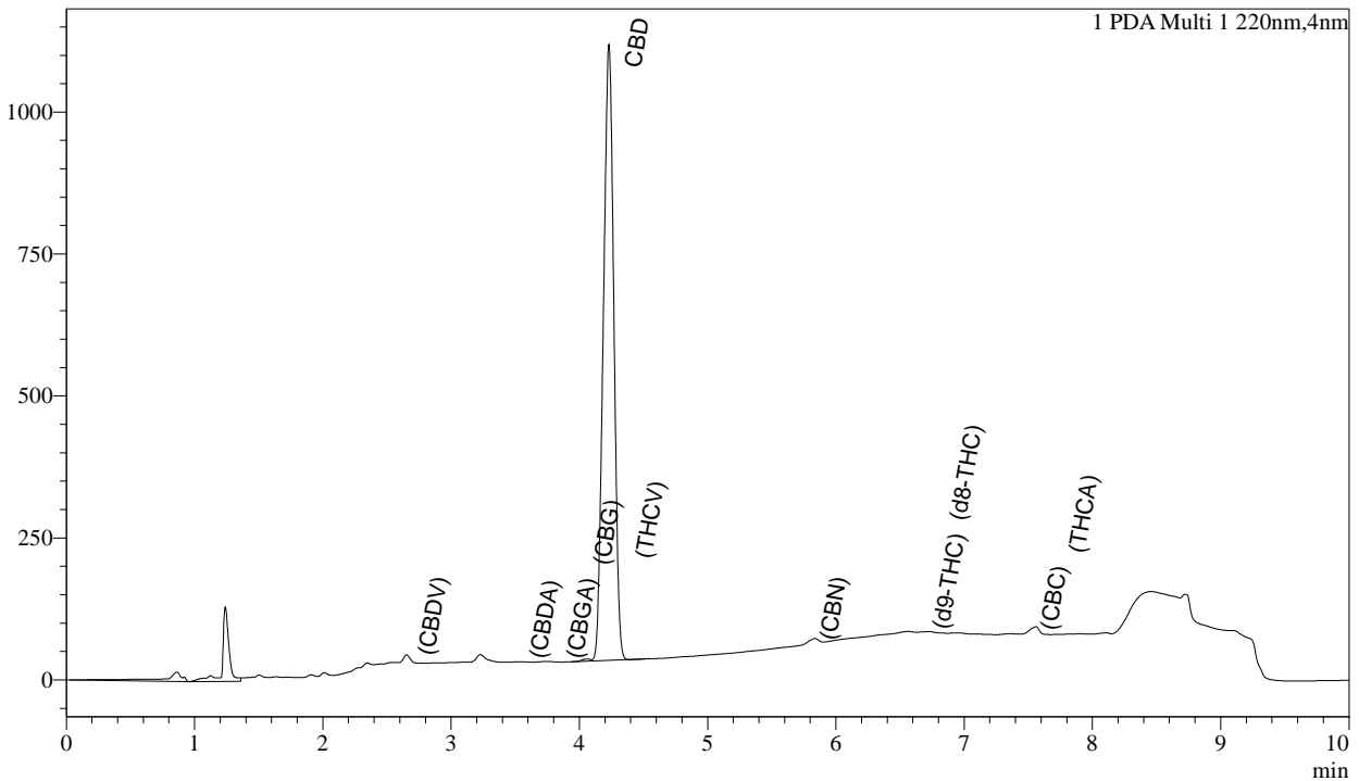
Chromatogram
