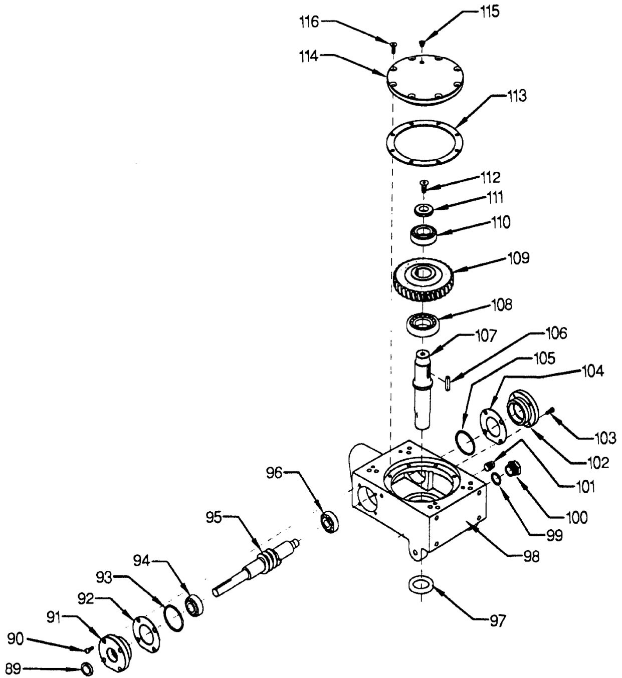
PARTS LIST 3
