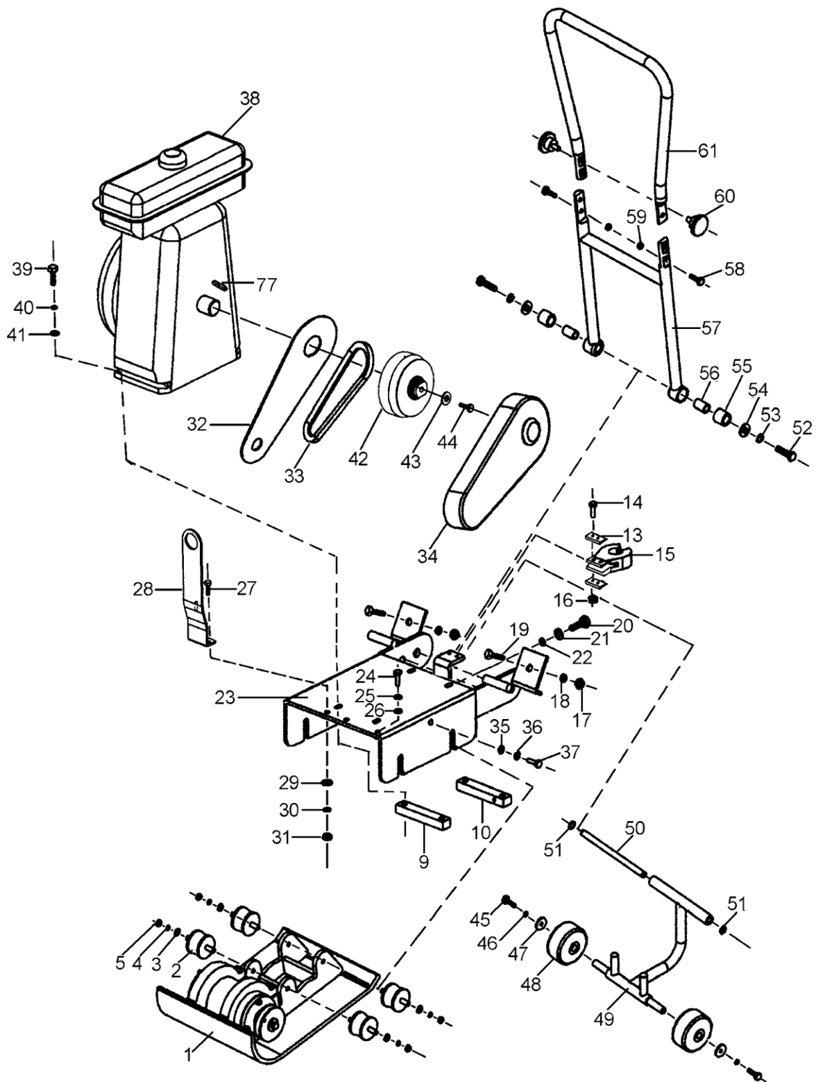
MS50 PARTS LIST 1
