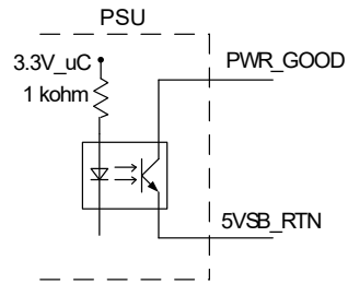
Fig. 14: Circuit diagram J3 Pin 9 (PWR_GOOD)
