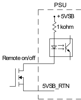
Fig. 13: Circuit diagram J3 Pin 10 (REMOTE ON/OFF)
