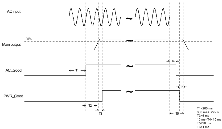
Fig. 16: Power Good/AC_Good function Timing
