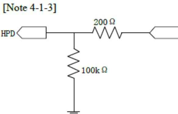
Fig.4-1-1 Equivalent circuit (Pin No.17)
