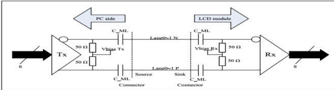
Fig.4-3-2 Main Link differential pair
