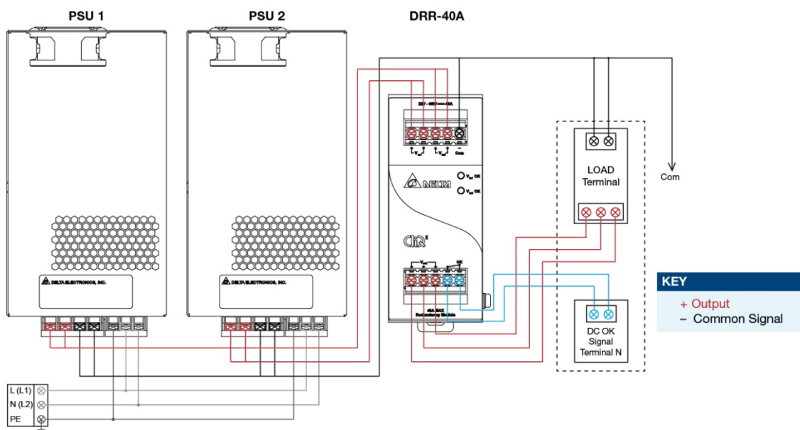
Fig. 3 Redundancy / Parallel Operation Connection Diagram
