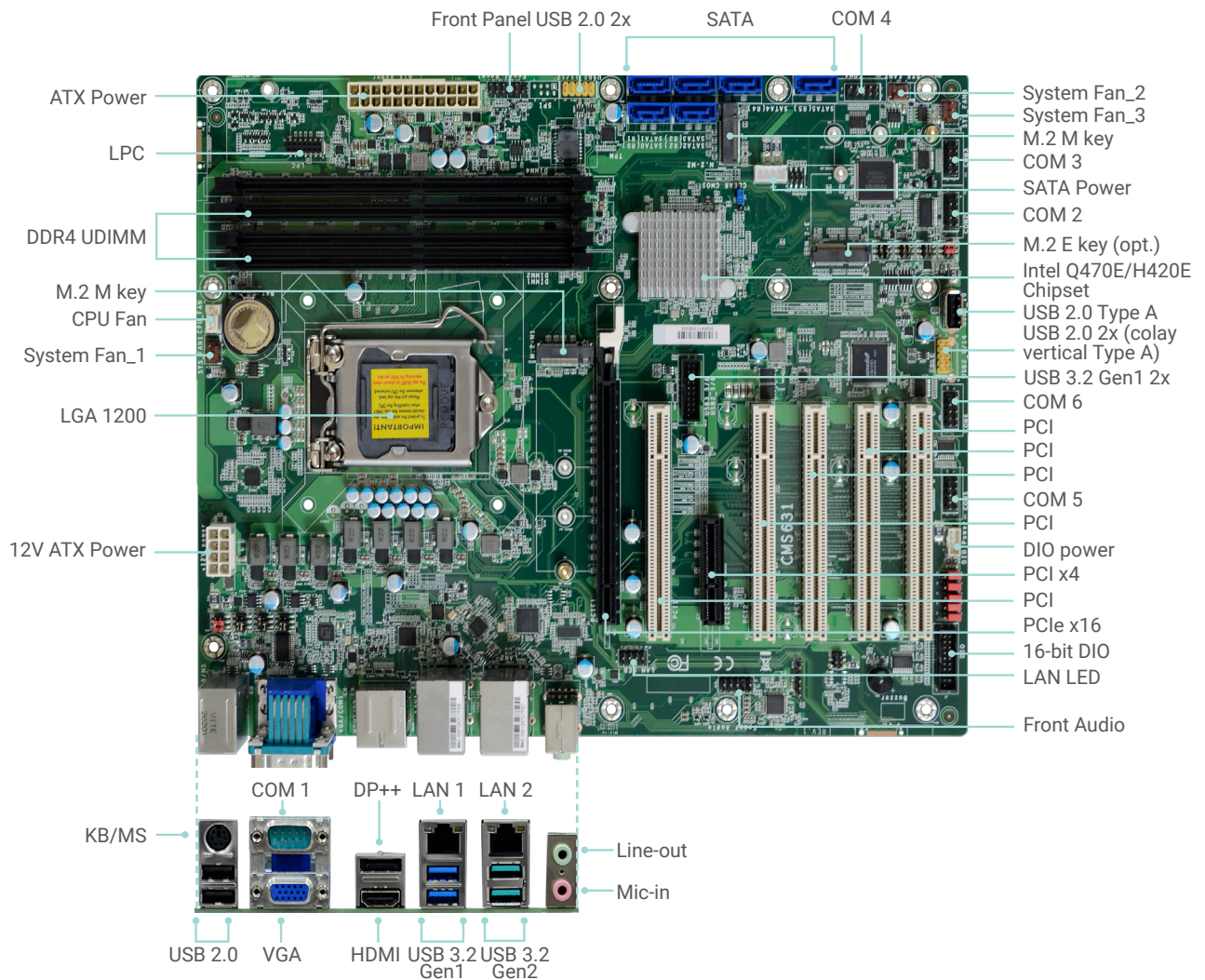
Top View
