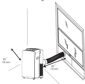
Vertical Sliding Window
