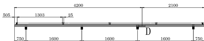
VISTA FRONTAL
