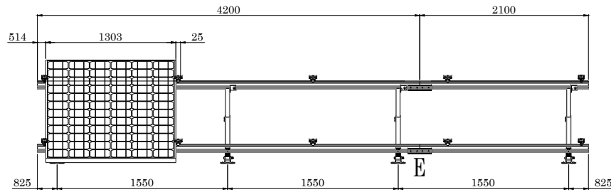
VISTA FRONTAL
