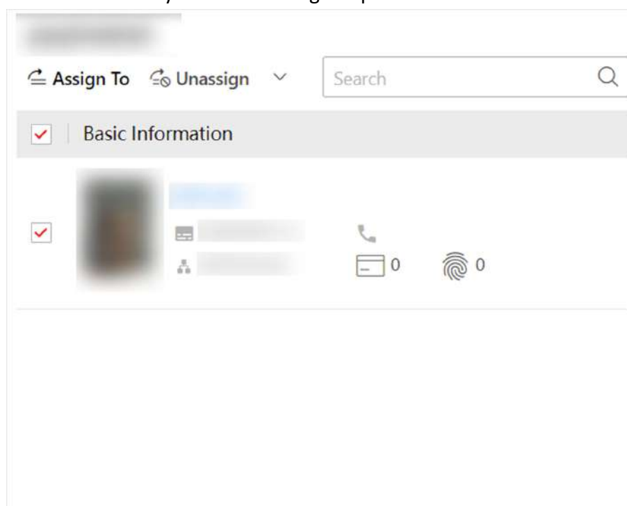
Figure 15-3 Assignee Panel
