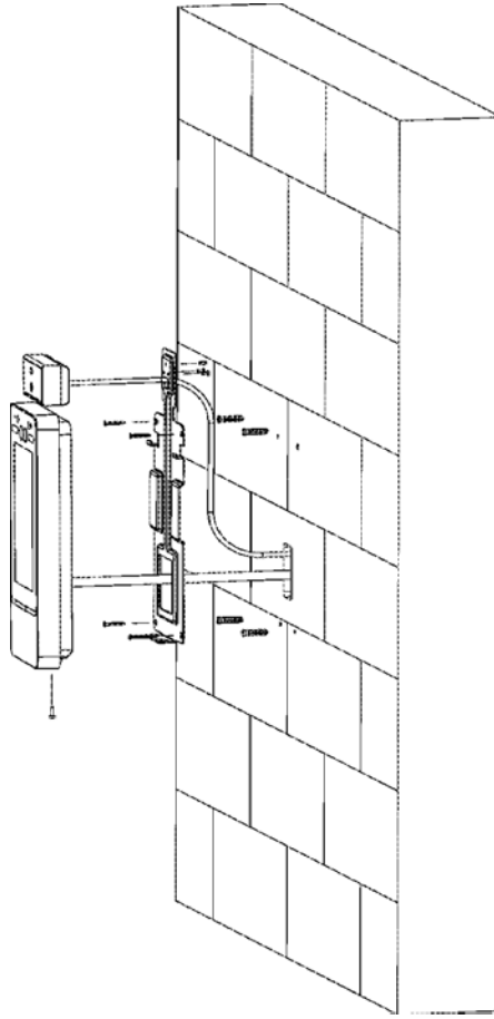
Figure 2-5 Installation diagram
