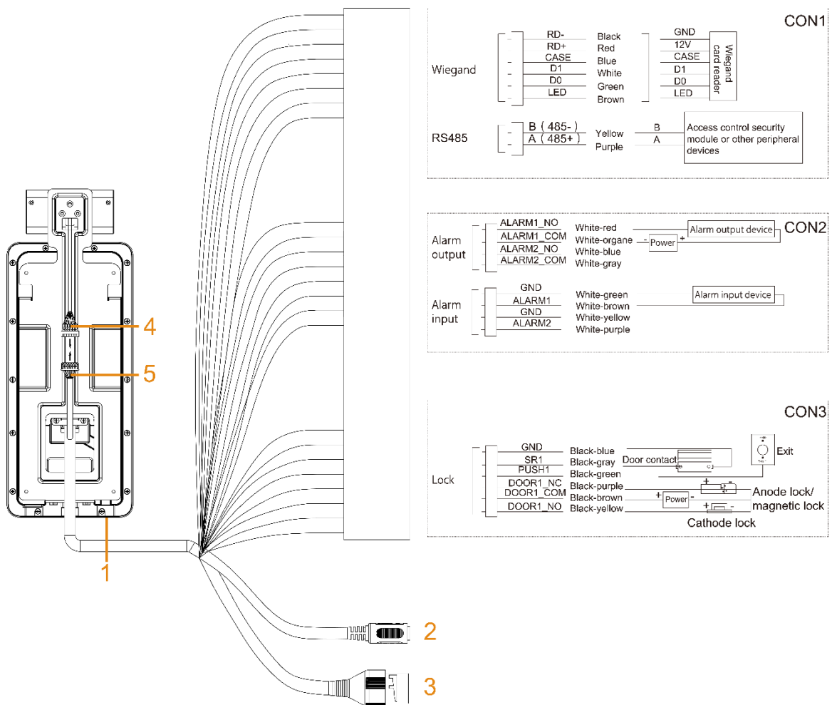
Figure 2-1 Cable connection
