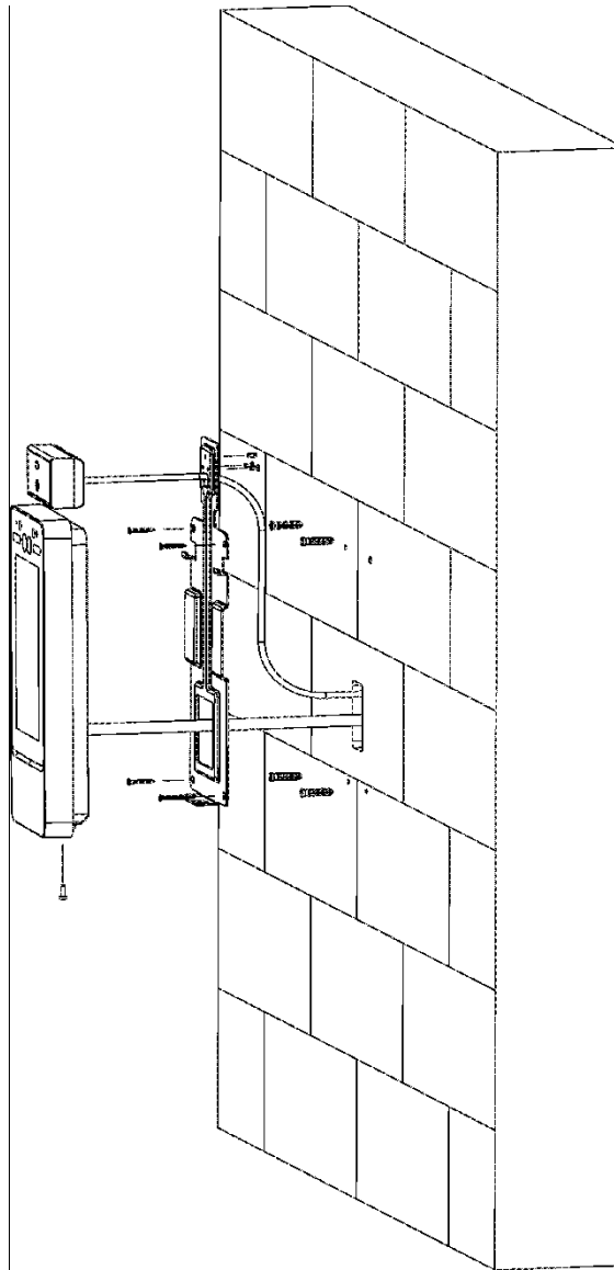
Figure 2-6 Installation diagram
