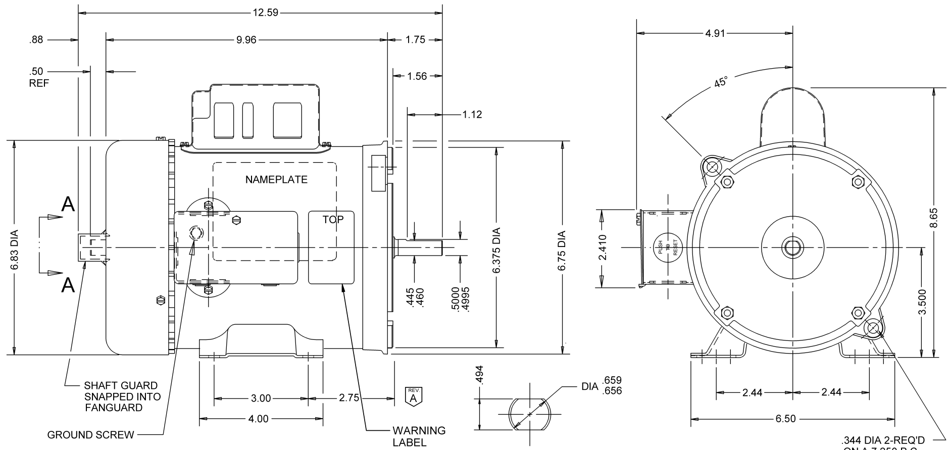
VIEW A-A (SHAFT GUARD NOT SHOWN FOR CLARITY) SCALE: 1/1
