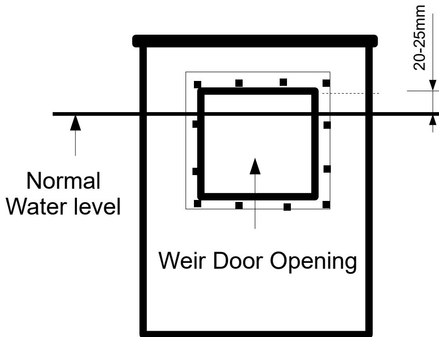
Skimmer Box Front view
