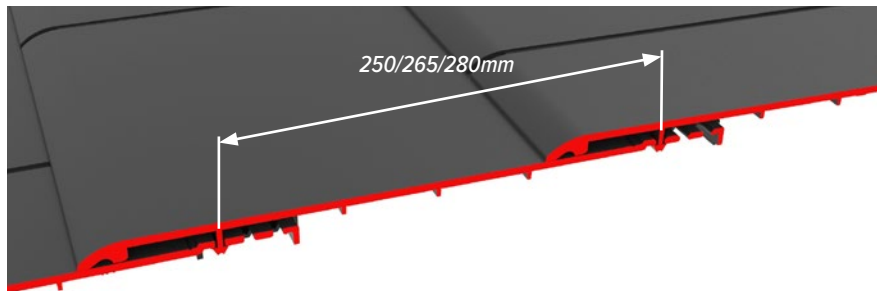
Ensure that you clip the tiles into the right slots depending on the batten gauge used.
