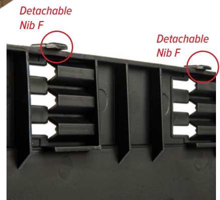
The nibs on the Envirotile raise the back of the tile off the roof face so maintaining a ventilation path.
