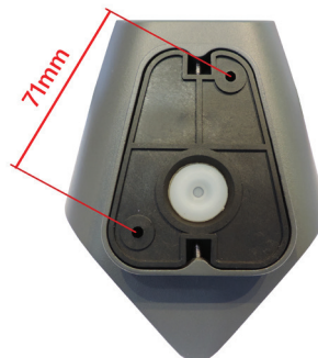
BACK PLATE
