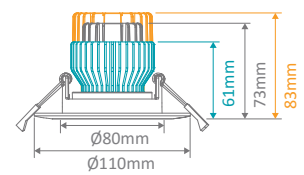
Cutout: Ø80-85mm Tilttable to 15°
