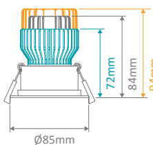
Cutout: Ø70-75mm
