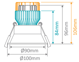
Cutout: Ø90-92mm DT90 Tilttable to 15°
