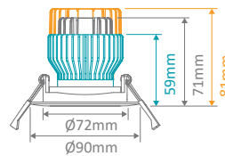
Cutout: Ø72-75mm Tilttable to 15°
