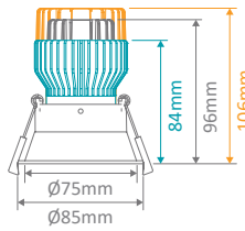
Cutout: Ø75-77mm
