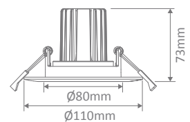
Cutout: Ø80-85mm
